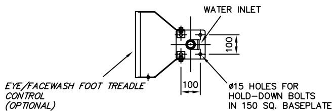
PLAN ON BASEPLATE
