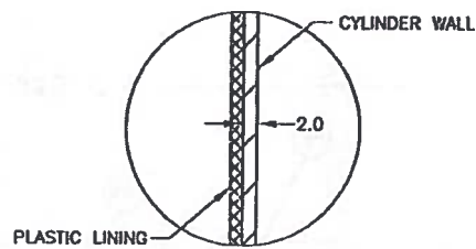
DETAIL FOR PLASTIC LINING
