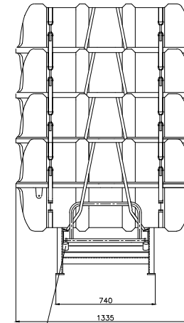
Holder for service pipe Place service pipe in holder while the raft is being lashed.
